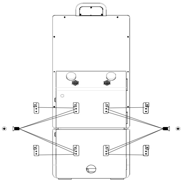
Step 1: Fix the 2pcs left and 2pcs right wall mount hooks onto the main system with 8pcs KM 4*6 screws (018.37.0059).
