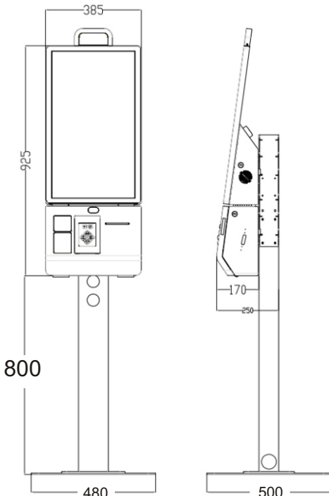
Lowest installation from the ground: 800mm
