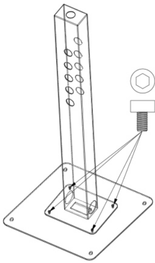
Step 2: Fix the column onto the base with 4pcs SHCS M6*12 screws(018.37.0018).
