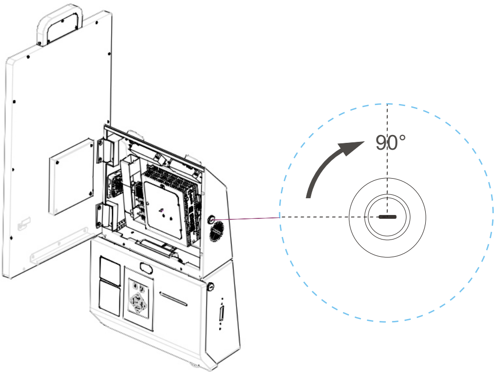
C. To unlock the main system door, insert the key and rotate it clockwise approximately 90 degrees, and the main system will open.
