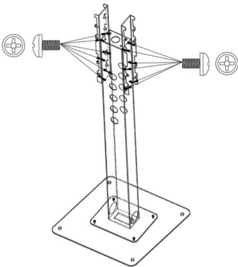
Step 3: Fix the 2 side brackets onto the column with 12pcs PM 5*12 screws (018.37.0105).
