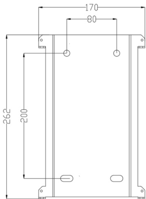
Wall Mount Bracket
