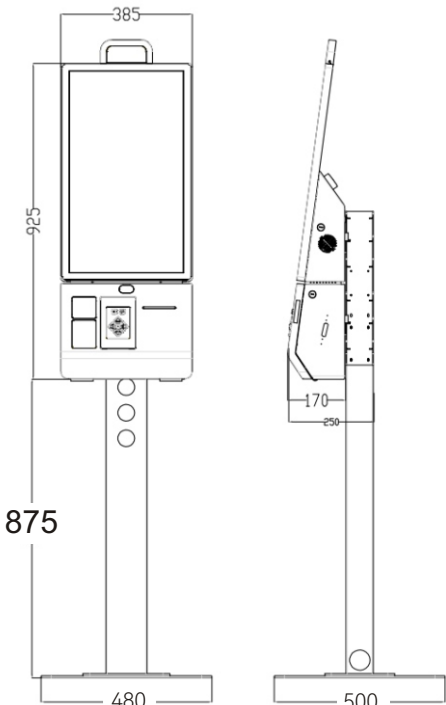
Medium installation from the ground: 875mm
