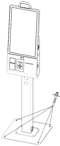
Step 5 (Optional): Secure the base to the floor with 4pcs M8*60 expansion bolts (018.37.0102) .
