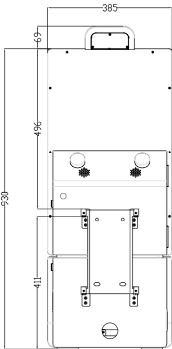
Main System And Wall Mount Bracket
